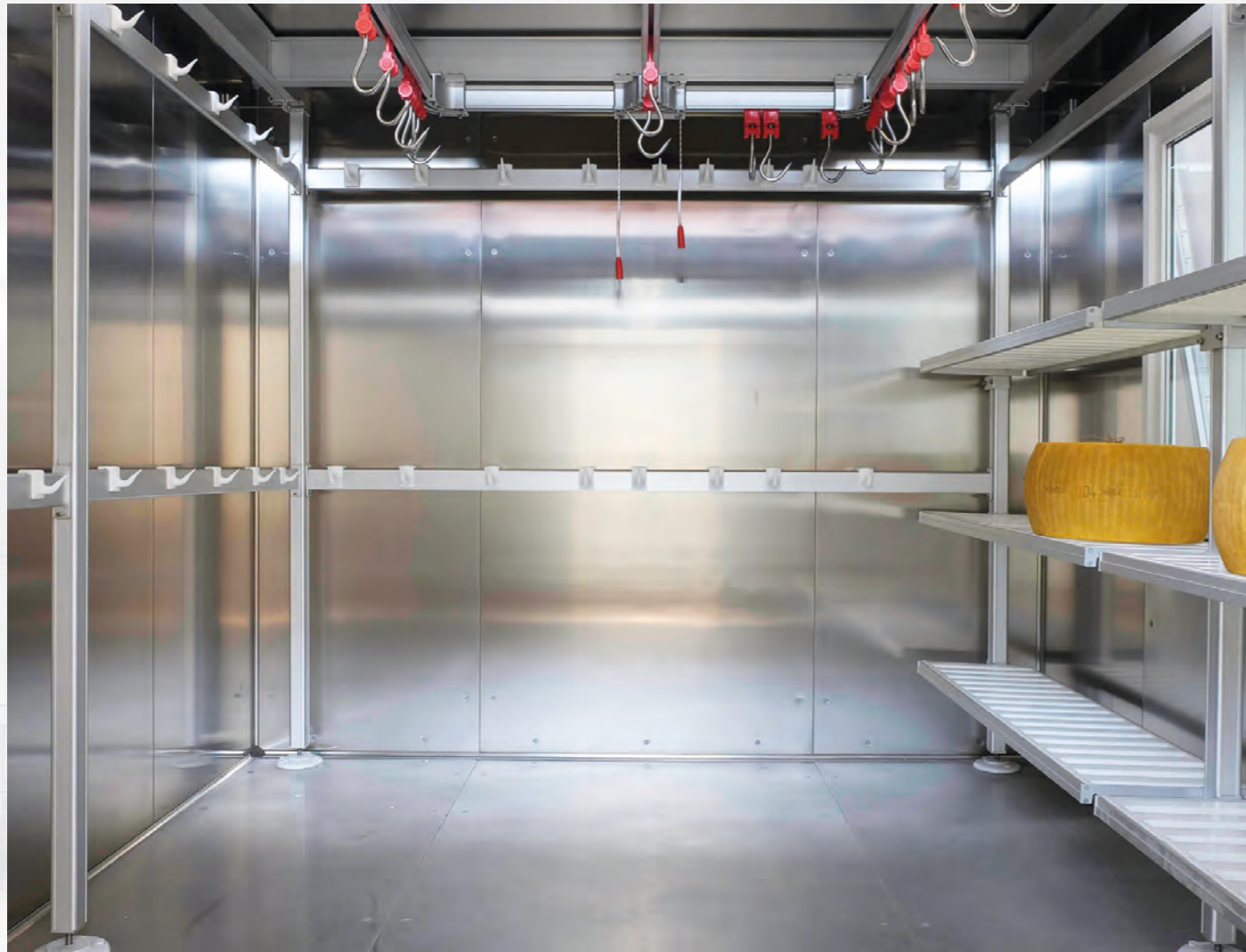
Celle con guidovia \ Cold rooms with rail passage
